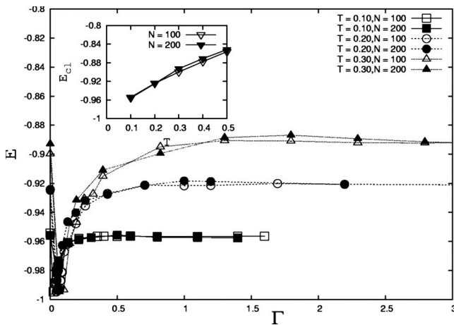
FIG. 3. Variation in average energy E with transverse field \Gamma for T=0.10, 0.20, and 0.30 ( h=0 ) for two different values of N ( N=100, 200 ). The corresponding average energies E_{cl} for various temperatures for N=100 and 200 are shown in the inset. E converges to the classical values E_{cl} for large \Gamma .
