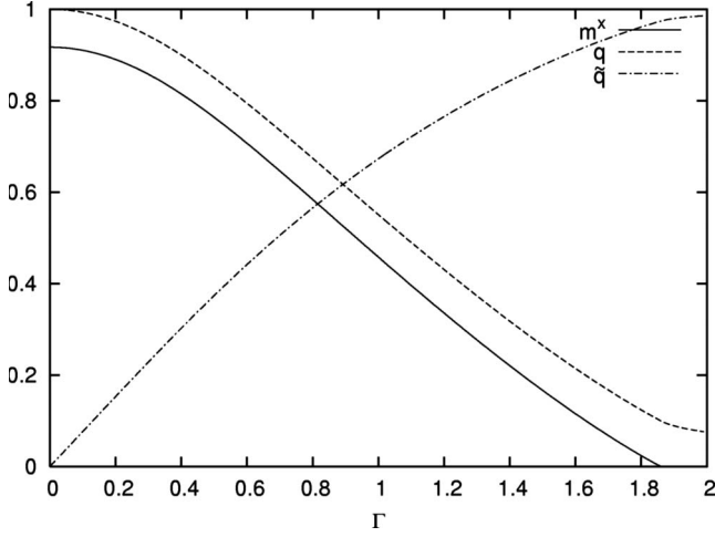
FIG. 7. Result of numerical calculations for the saddle-point equations for m_x , q , and \tilde{q} as a function of \Gamma for T \neq 0 .
